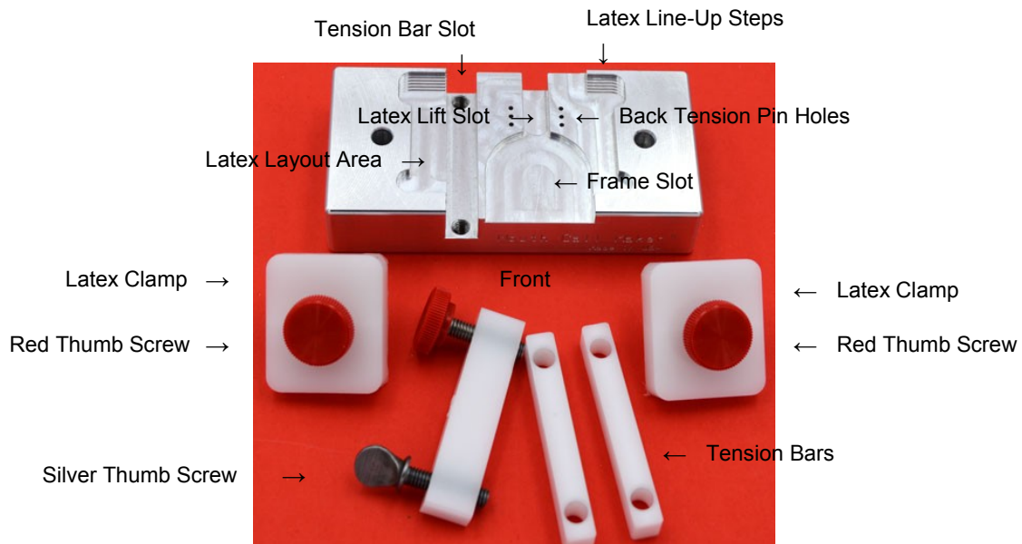
Mouth Call Maker™ Jig with Part Names
